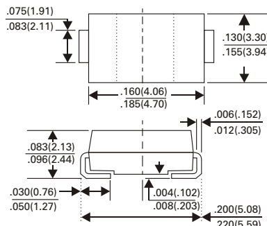
SMB/DO-214AA
