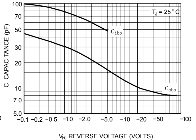
Figure 3. Capacitance
